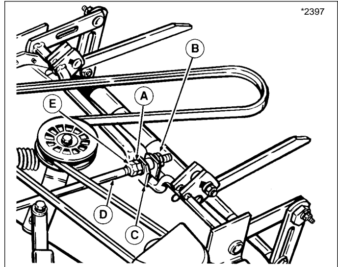
Figure 33. Front-To-Back Levelling
