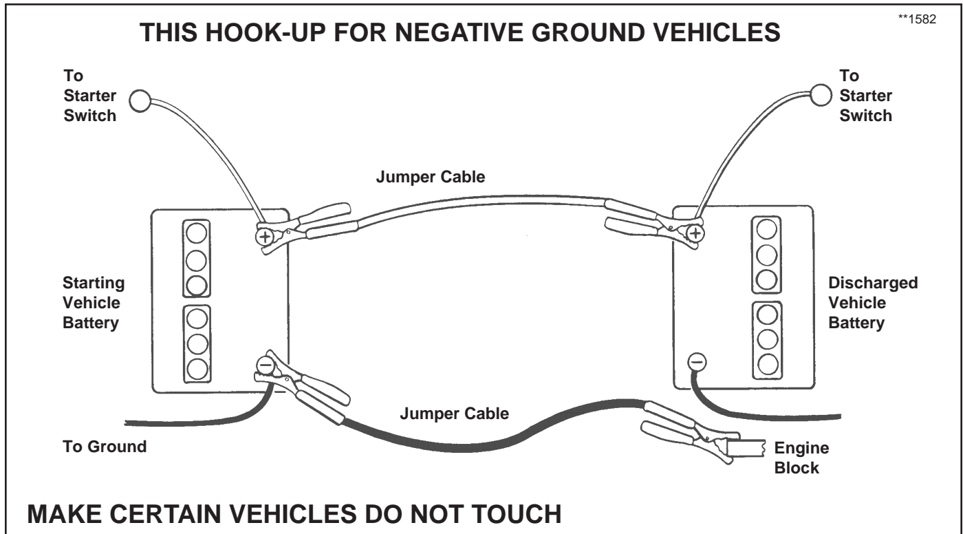
Figure 23. Battery Jump Starting Diagram
