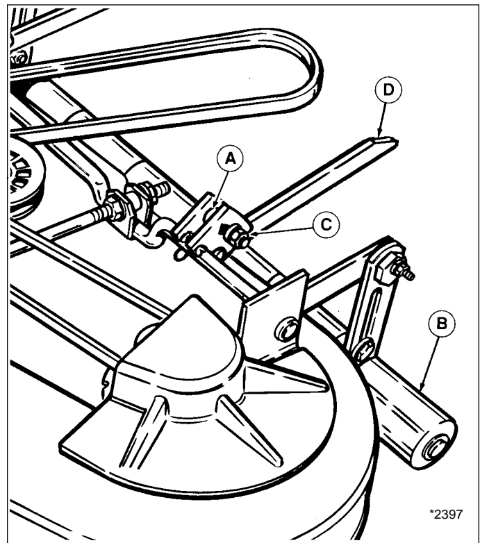
Figure 34. Transport Height Adjustment
