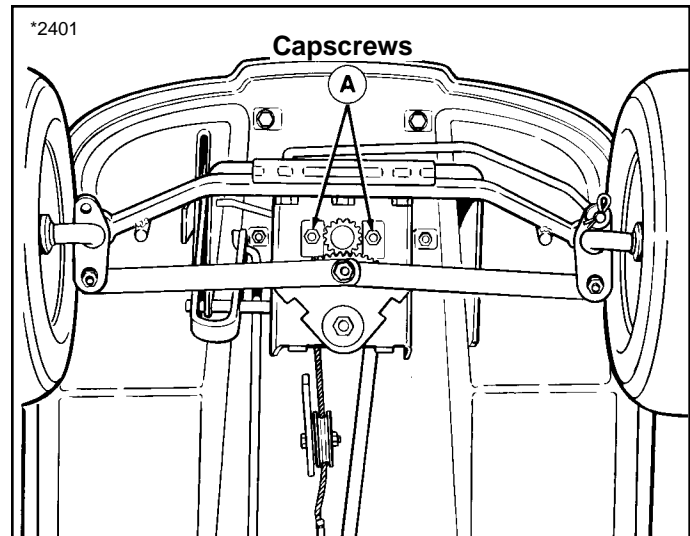
Figure 30. Steering Gear Adjustment
