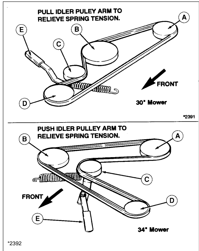
Figure 6. Mower Belt Pattern
