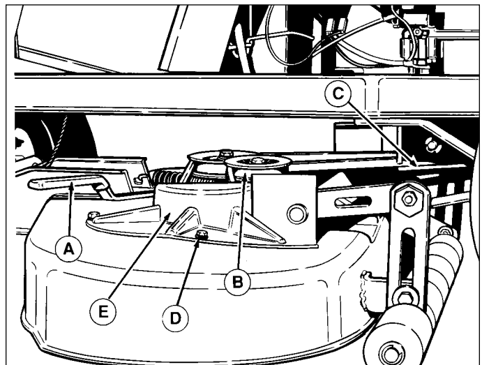
Figure 36. Mower Belt Replacement - 34"
