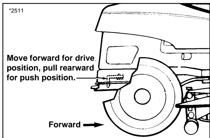
Figure 12. Transaxle Release Lever - Hydro Models
