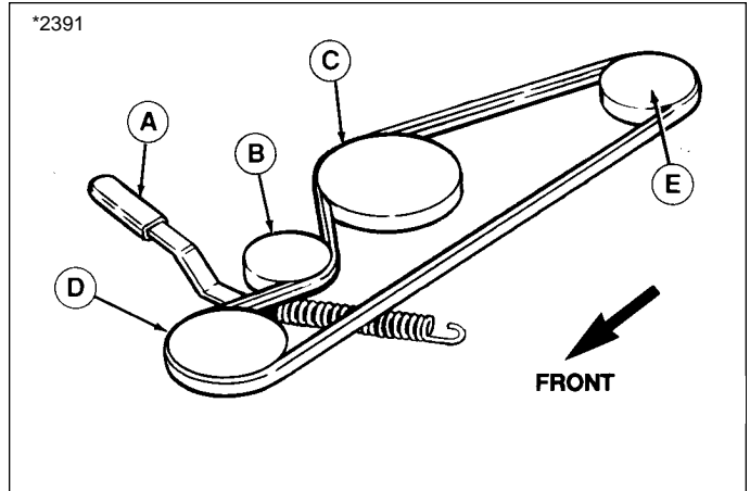
Figure 35. Belt Pattern - 30" Mower
