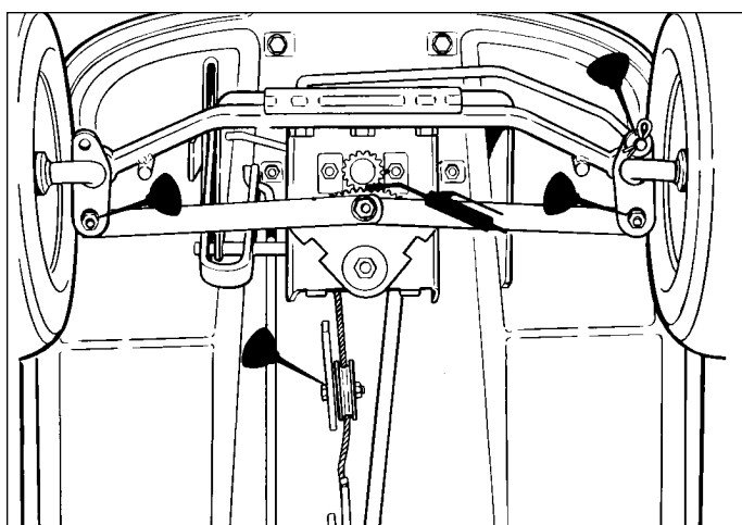
Figure 14. Rider Lubrication Points - Front Half
