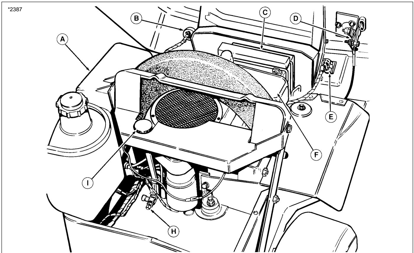
Figure 3. Engine Compartment
