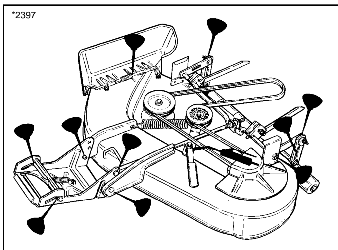
Figure 15. Front Axle Lubrication Points
