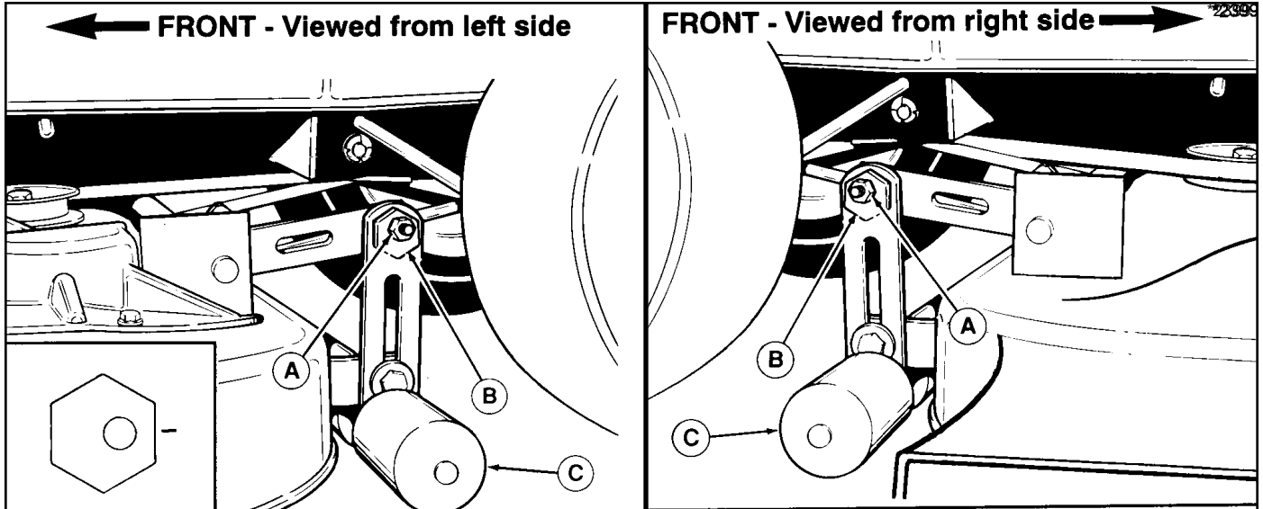
Figure 31. Leveling The Mower Side-to-Side
