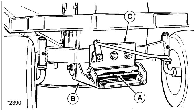
Figure 6. Mower Hitch
