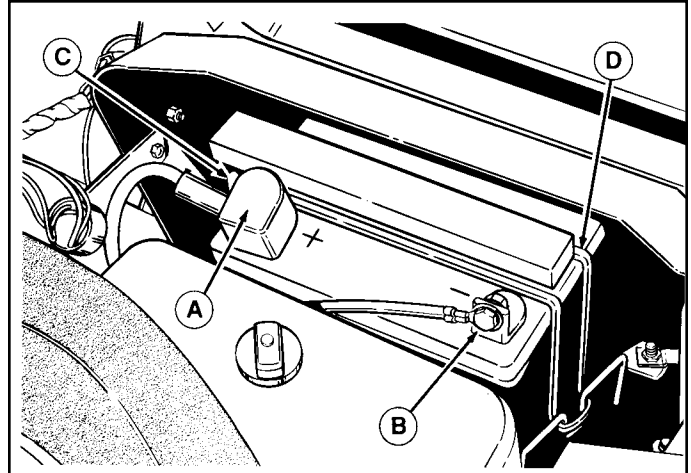
Figure 19. Battery A. Positive Battery Terminal C. Vent Tube B. Negative Battery Terminal D. Holddown Strap
