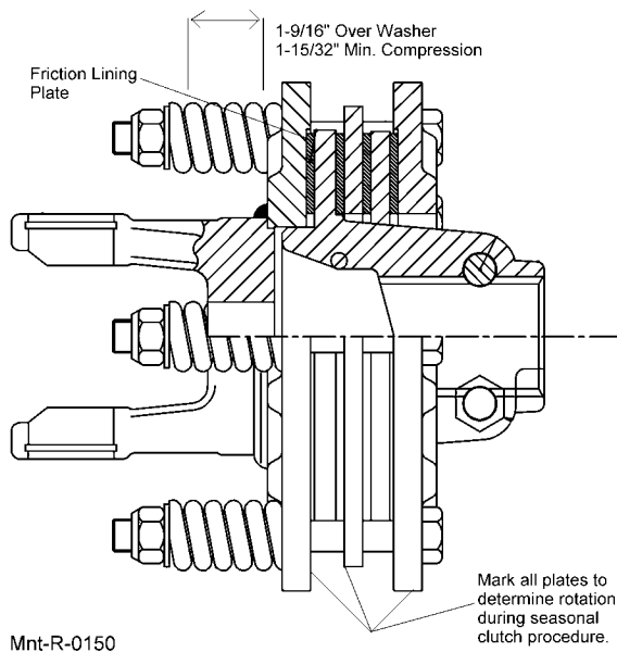
Coil Spring Slip Clutch (1) Intermediate Drive
