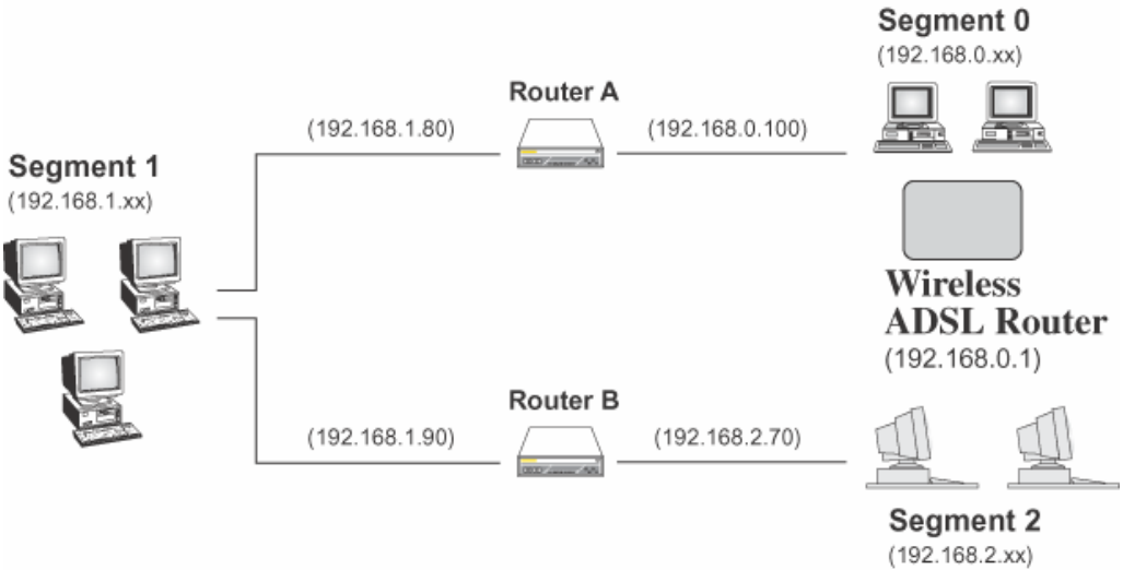
Figure 75: Routing Example
