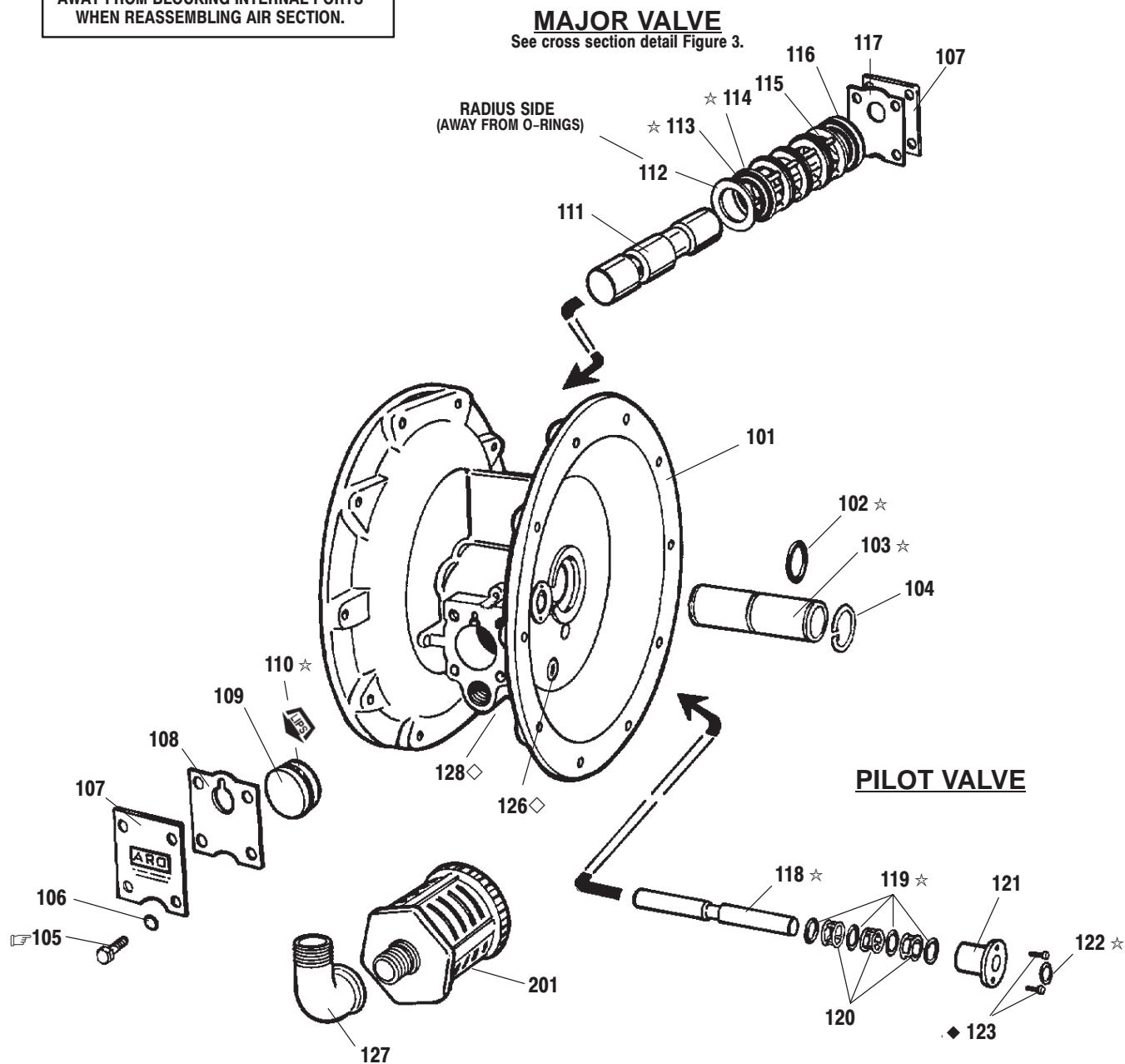
MAJOR VALVE CROSS SECTION DETAIL
