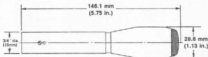
FIGURE 2 — Dimensions
