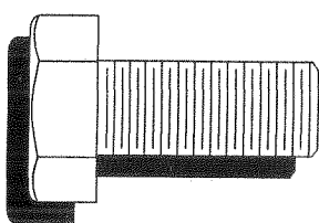
(1) Hex Bolt 1/2-13 x 1
