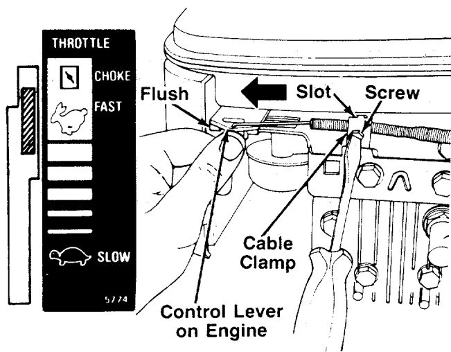
FIGURE 6C.—Models 466R, 469R, 476R and 479R
