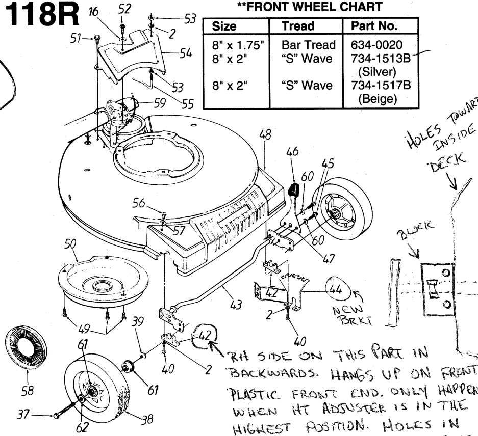
PARTS LIST FOR MODELS 115R AND 118R ROTARY MOWERS
