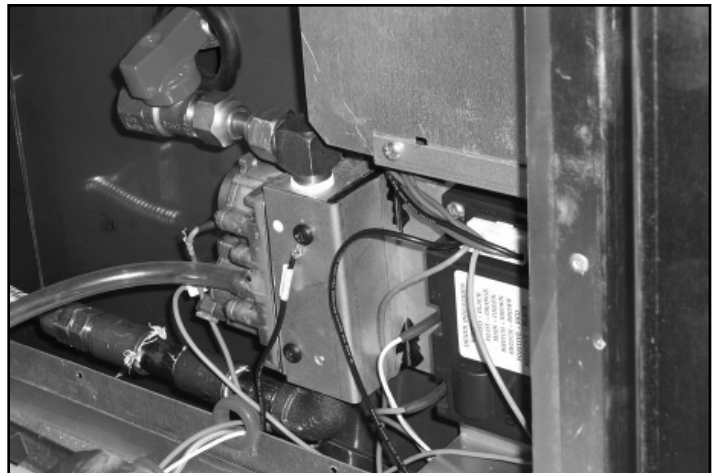
Figure 6.6 Connect Manometer
