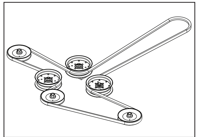
Belt routing
