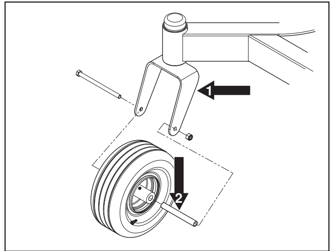
Caster wheels
