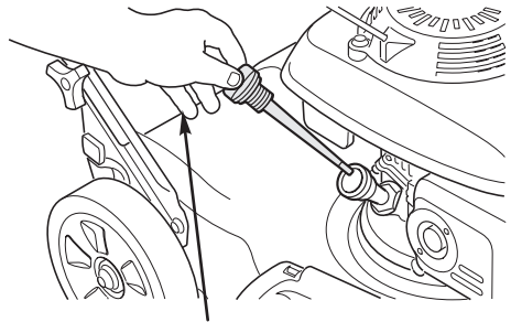
FILLER CAP/DIPSTICK
