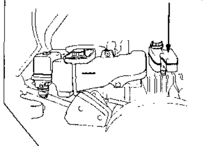
TRANSMISSION FLUID RESERVOIR (H3011H HYDROSTATIC TRANSMISSION)
