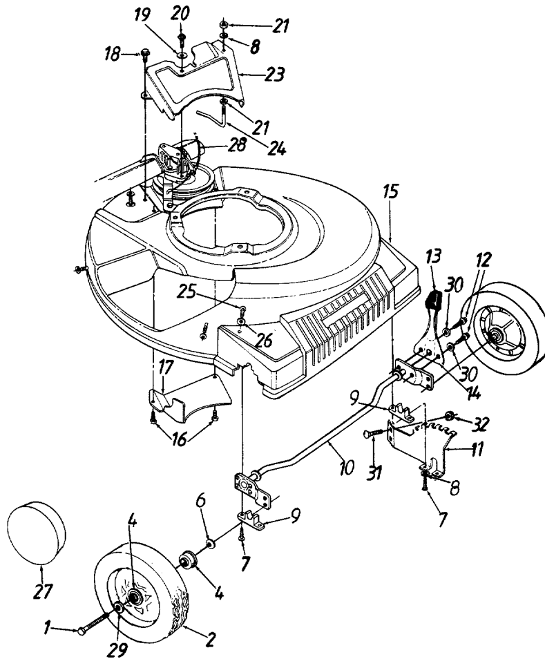
PARTS LIST FOR MODEL 123E898E ROTARY MOWER
