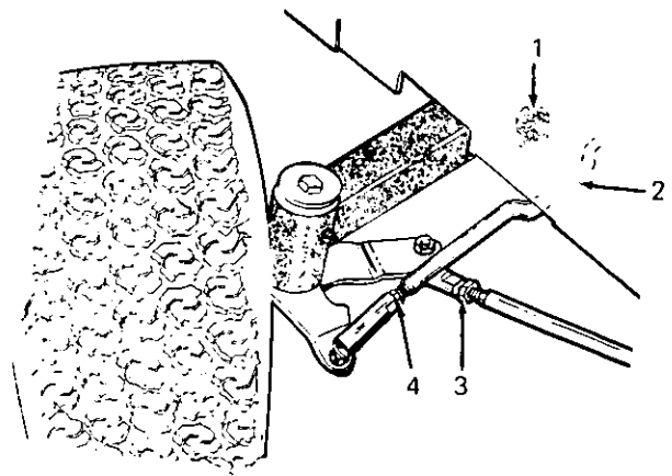
Figure 24 Tie Rod and Drag Link Ball Joints
