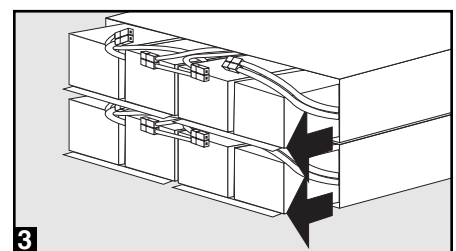
3 Remove Internal Batteries (Slide From Battery Pack Cabinet)
