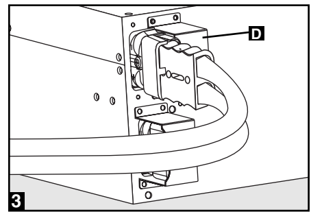
3 Attach the retention brackets D to the right of each connector, using the preexisting holes set to the right of the original bracket position.
