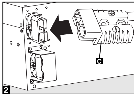
2 Insert one end C of the detachable power cable into each connector. (See the UPS manual for the external battery connector description and location.)
