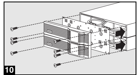
10 Restore Battery Cover Plate and Battery Pack Front Panel (Screw Into Place)
