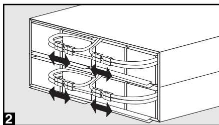
2 Disconnect Internal Batteries (4 Sets of Red/Black Connectors)
