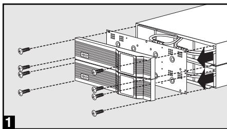
1 Unscrew and remove Battery Pack Front Panel and Battery Cover Plate
