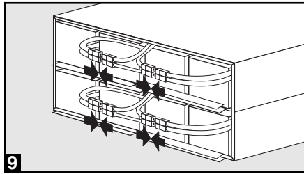
9 Connect 4 Sets of Red/Black Internal Battery Connectors (Connect Black to Black and Red to Red.)
