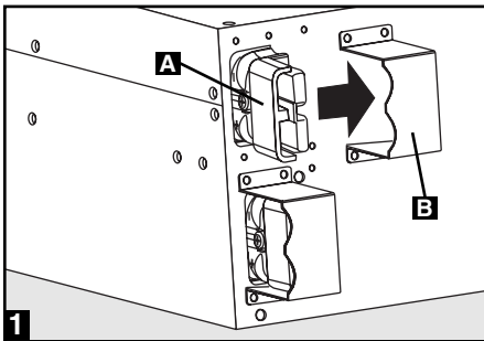
1 Remove the retention brackets B from the UPS system power module's external battery pack connector and one of the battery pack's rear panel connectors A .
