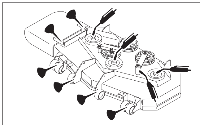
Figure 21. Deck Lubrication
