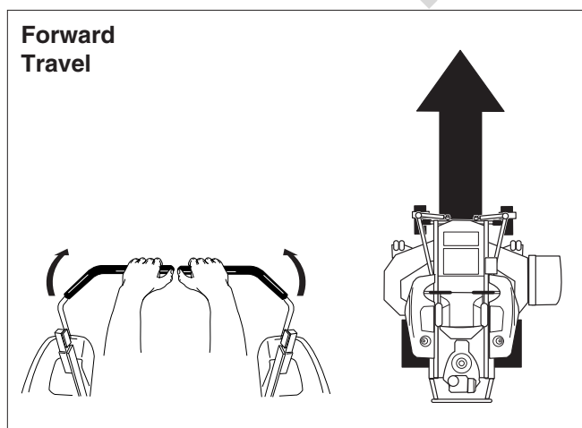
Figure 11. Forward Travel
