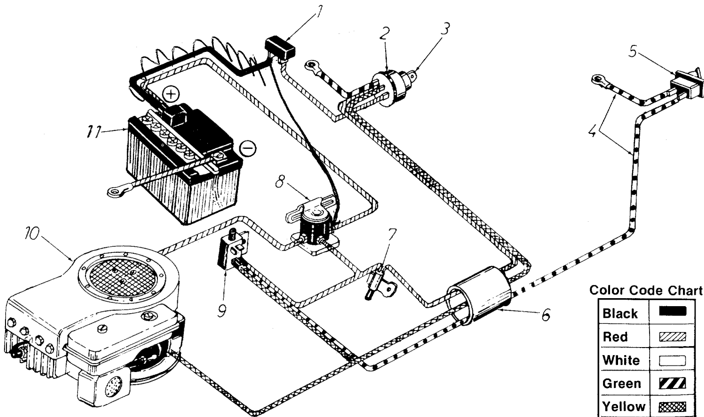
PARTS LIST FOR ELECTRICAL SYSTEM RIDING MOWER MODEL 525 ONLY
