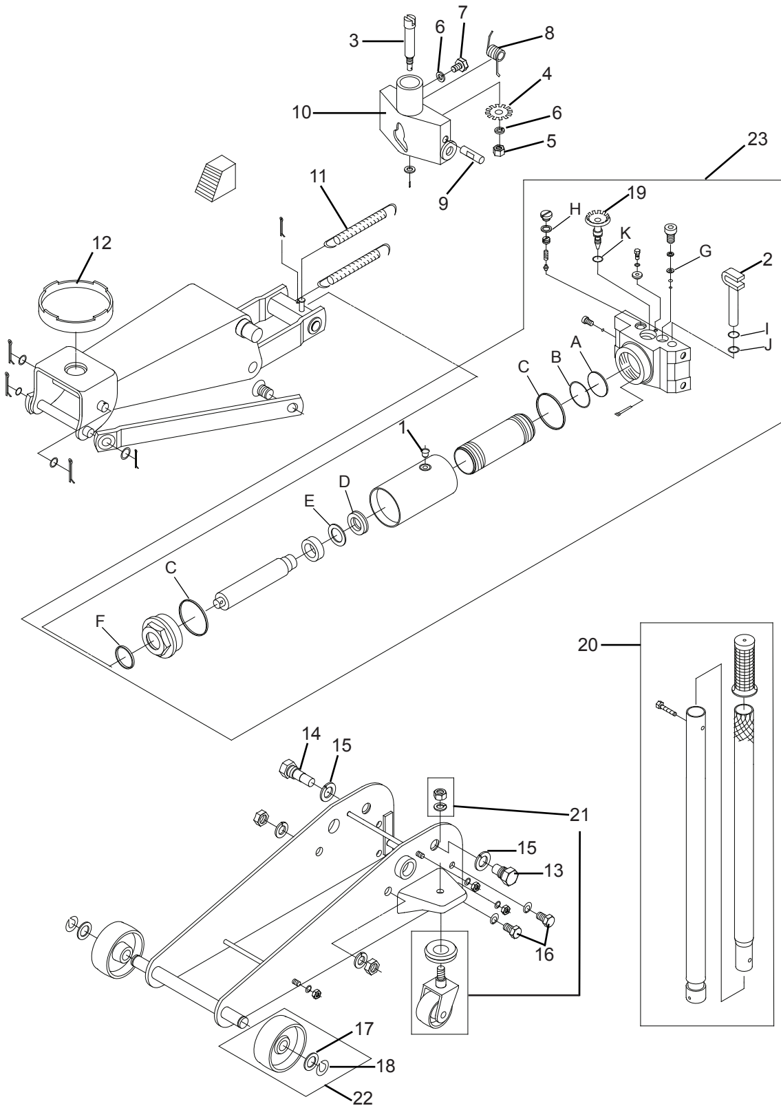
Figure 2 - Replacement Parts Illustration for Model Atd-7333
