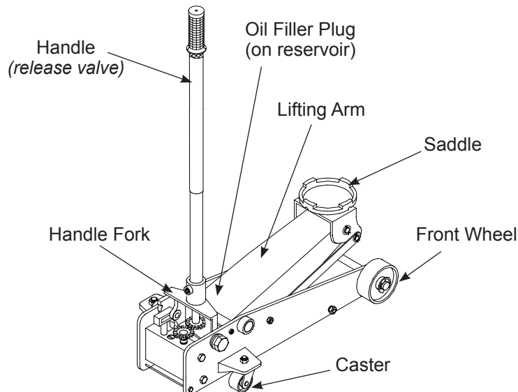
Figure 1 - Typical Service Jack Nomenclature
