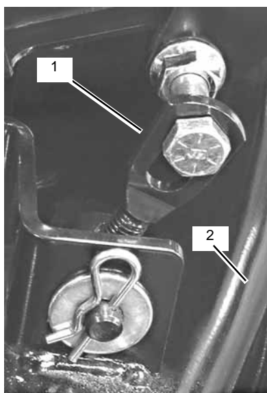
1. Trunnion 2. Mower Deck
