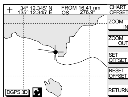
Plotter display, chart offset selected
