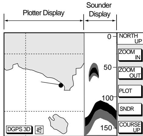
Plotter/Sounder display
