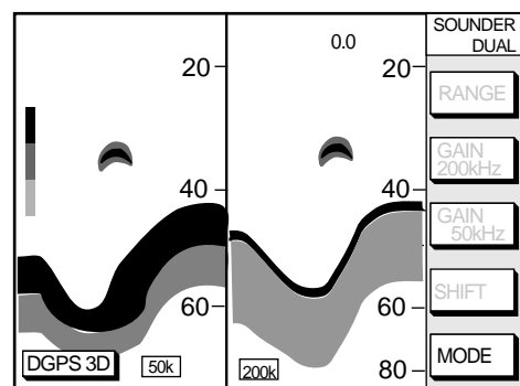
Dual-frequency display example
