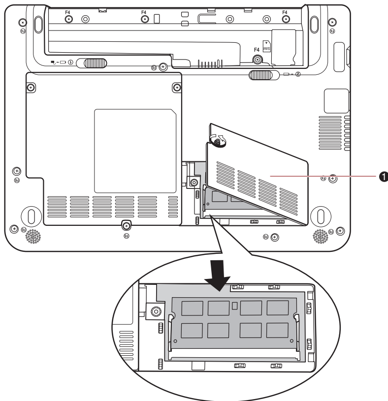
Figure 8-2 Removing the memory module cover
