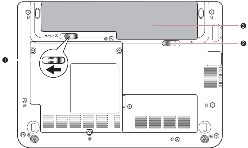
Figure 6-1 Releasing the battery pack (1)
