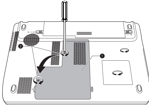
Figure 3-13 Seating the memory module cover
