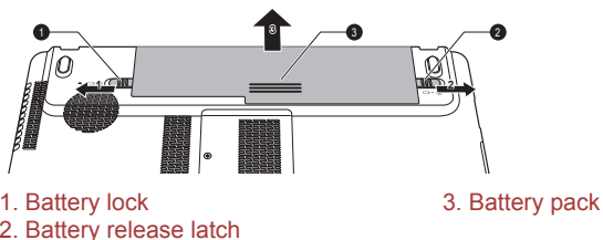
Figure 5-1 Releasing the battery pack
