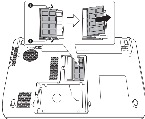
Figure 3-14 Removing the memory module
