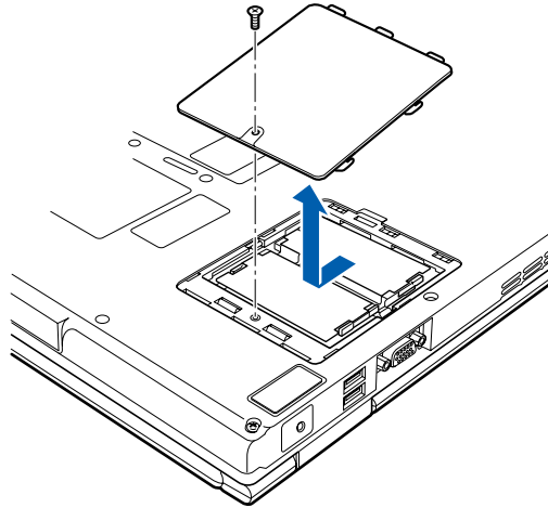
Figure 28. Opening the Memory Compartment
