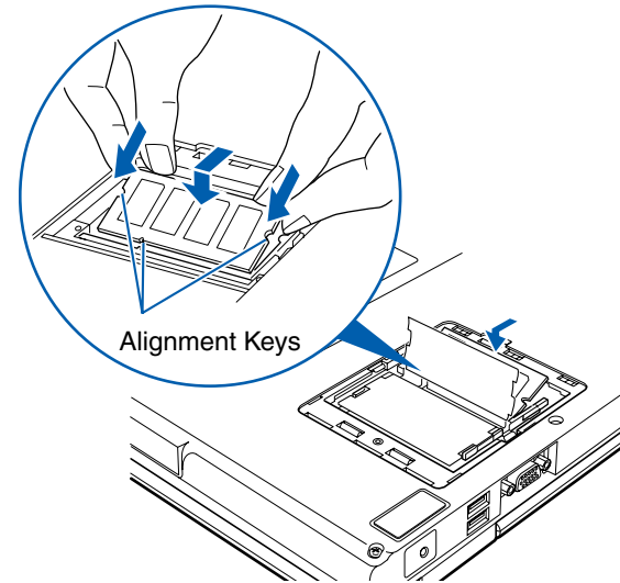
Figure 29. Installing a Memory Module
