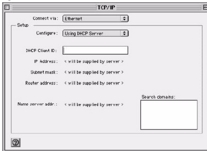
Figure 76 Macintosh OS 8/9: TCP/IP
