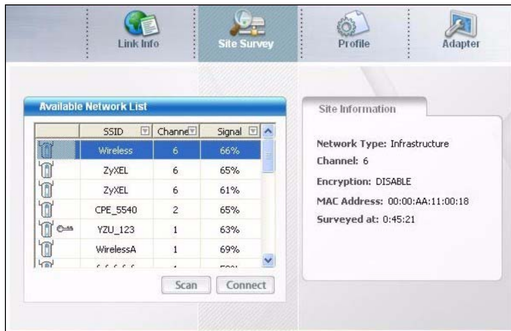
Figure 24 Station Mode: Site Survey
