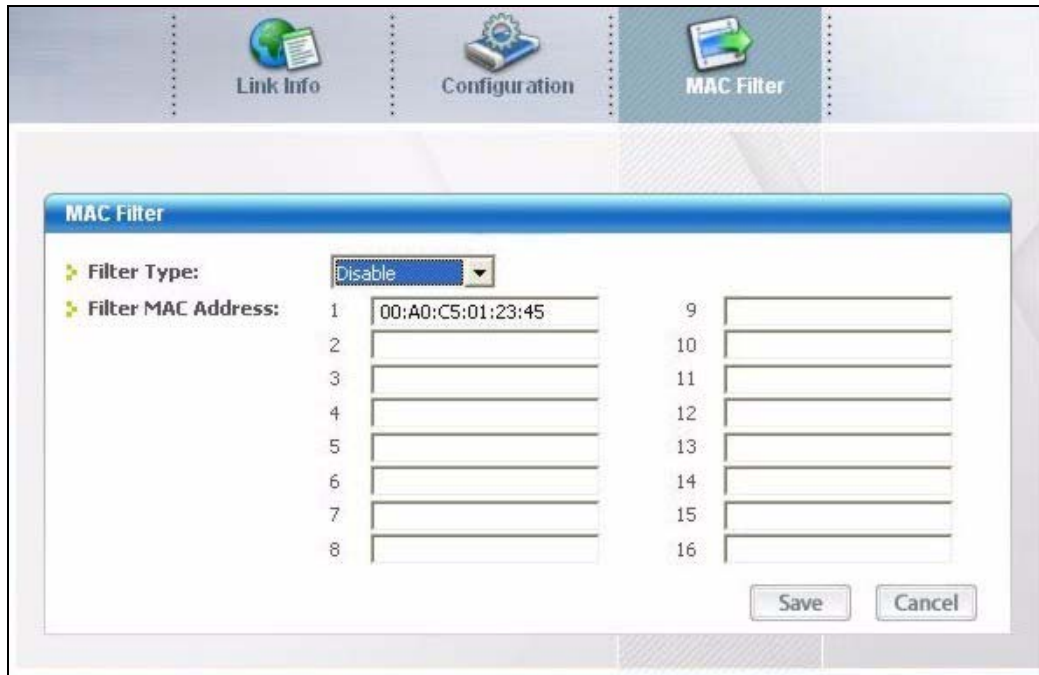
Figure 41 Access Point Mode: MAC Filter
