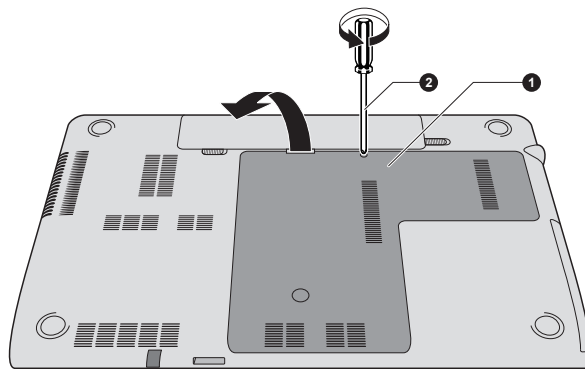
Figure 3-12 Removing the memory module cover
