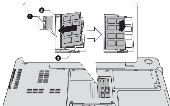
Figure 3-13 Seating the memory module
