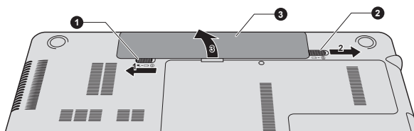
Figure 5-1 Releasing the battery pack -1
