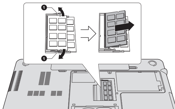
Figure 3-15 Removing the memory module
