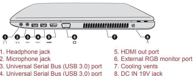
Figure 2-3 The right side of the computer
