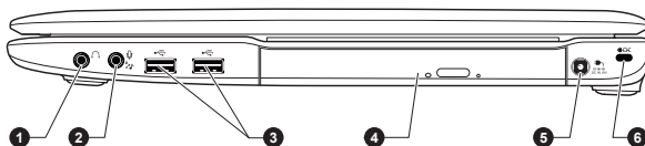
Figure 2-3 The right side of the computer
