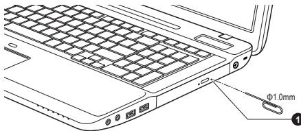
Figure 3-7 Manual release with the eject hole
