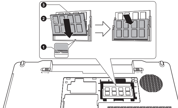
Figure 3-12 Seating the memory module
