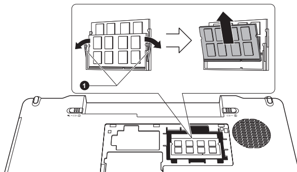
Figure 3-14 Removing the memory module
