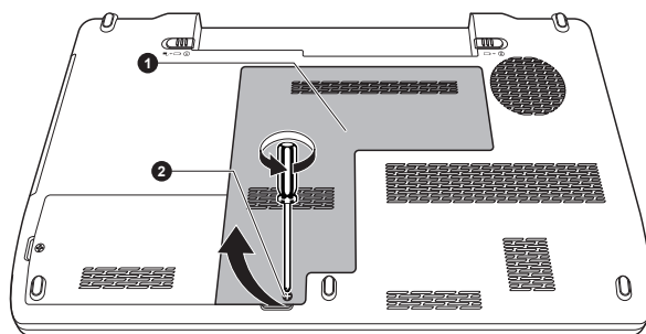
Figure 3-11 Removing the memory module cover
