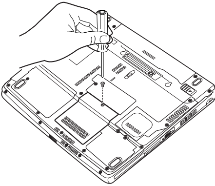
Memory module slot cover
