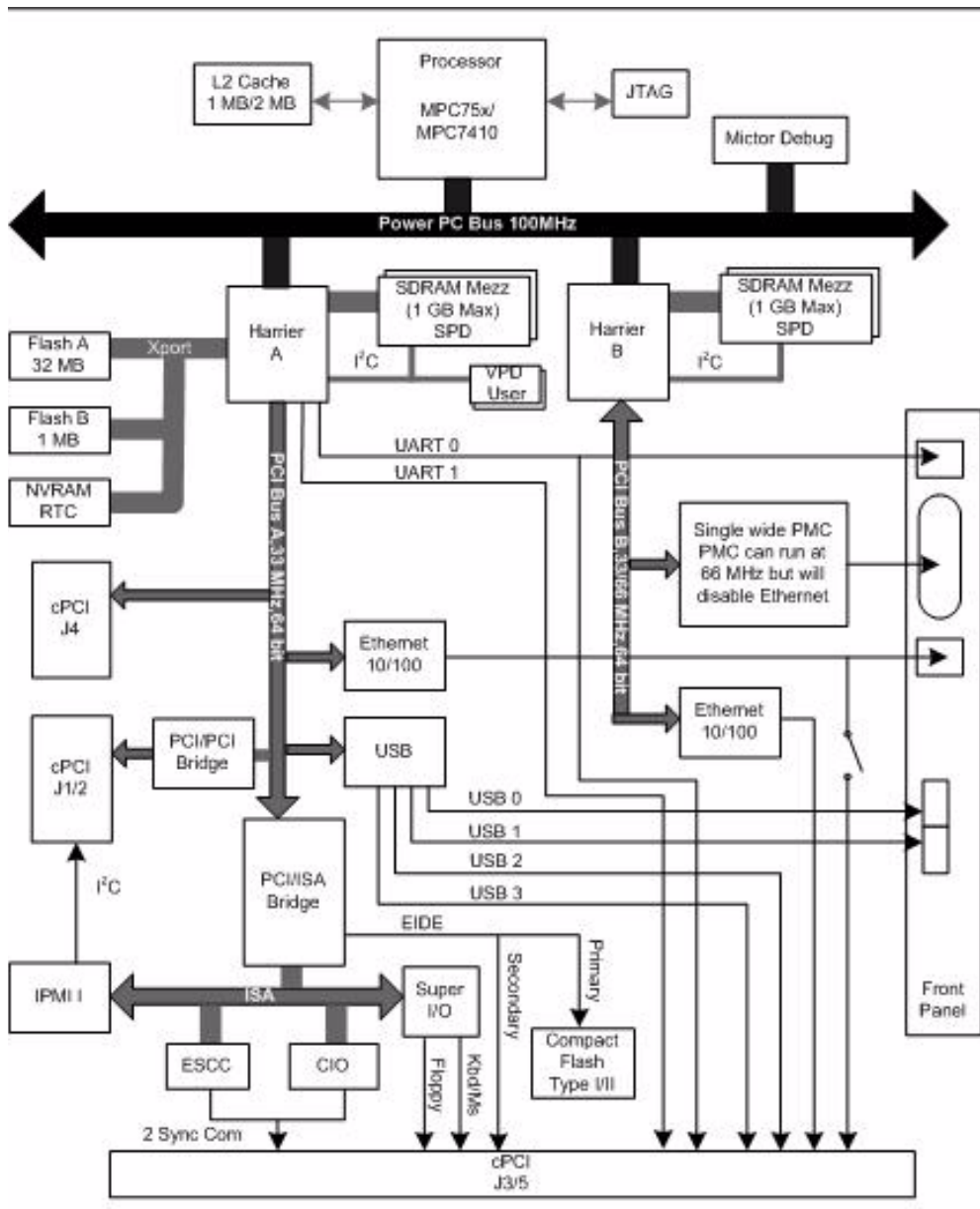
Figure 4-1 Block Diagram
