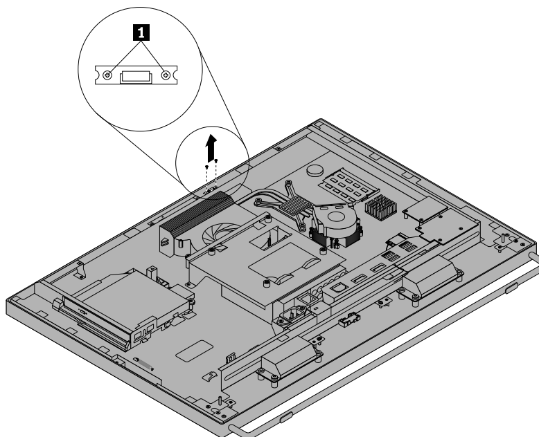
Figure 37. Removing the ambient light sensor
