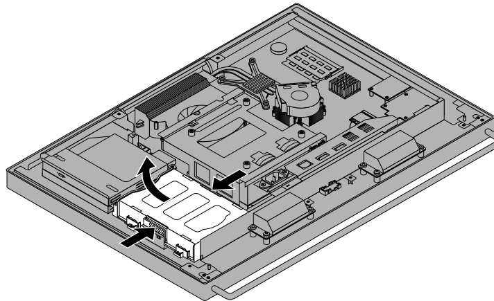
Figure 18. Removing the hard disk drive (20-inch display)
