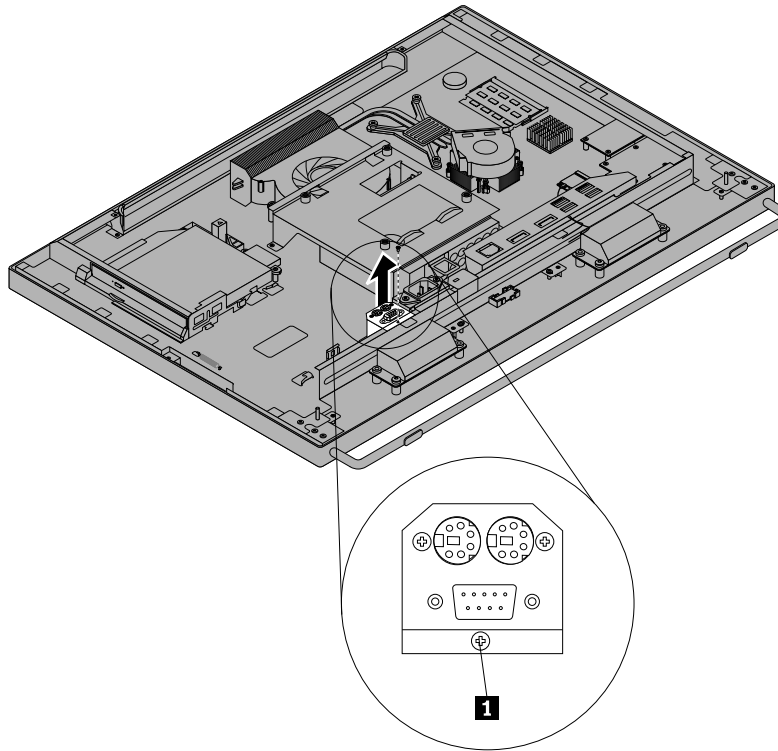
Figure 42. Removing the rear PS/2 connectors and serial port assembly
