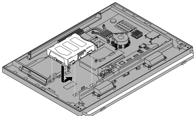
Figure 22. Installing the hard disk drive (23-inch display)
