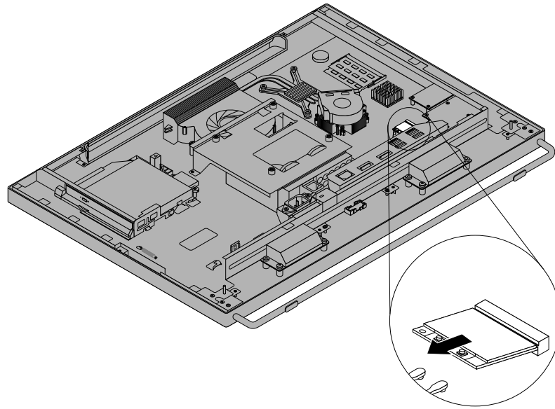
Figure 36. Removing the WI-FI card
