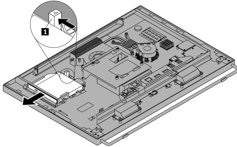
Figure 23. Removing the optical drive
