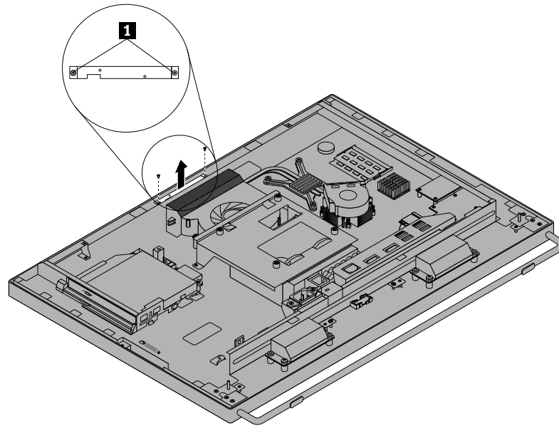
Figure 34. Removing the integrated camera
