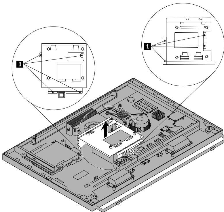
Figure 31. Removing the VESA mount bracket
