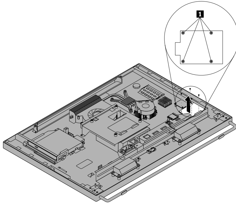
Figure 40. Removing the ExpressCard
