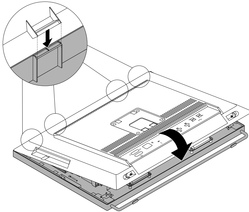
Figure 46. Installing the computer cover
