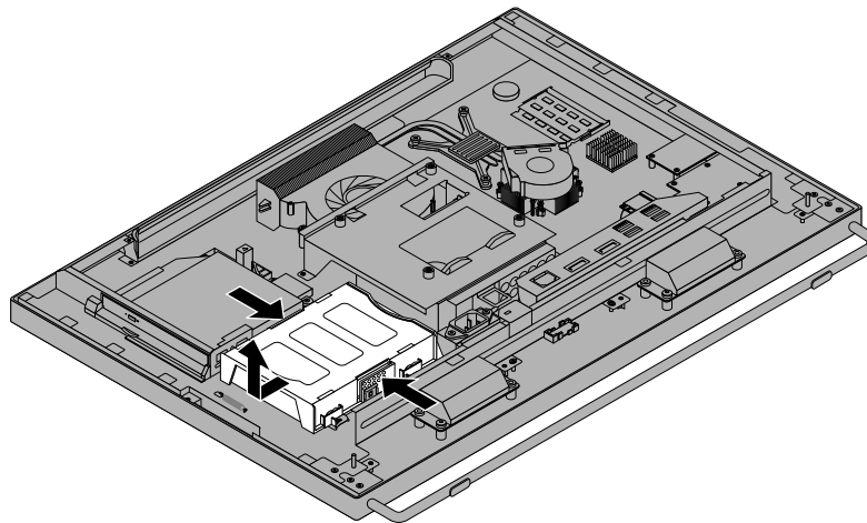
Figure 19. Removing the hard disk drive (23-inch display)
