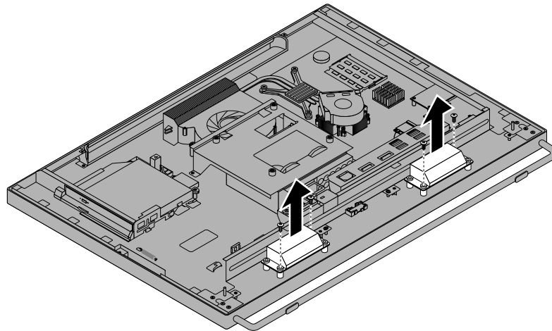
Figure 30. Removing the internal speakers
