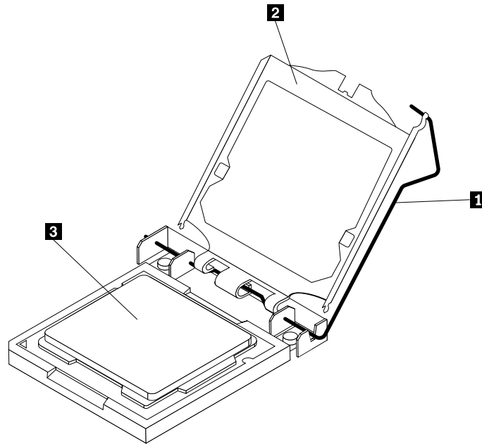
Figure 27. Accessing the microprocessor
