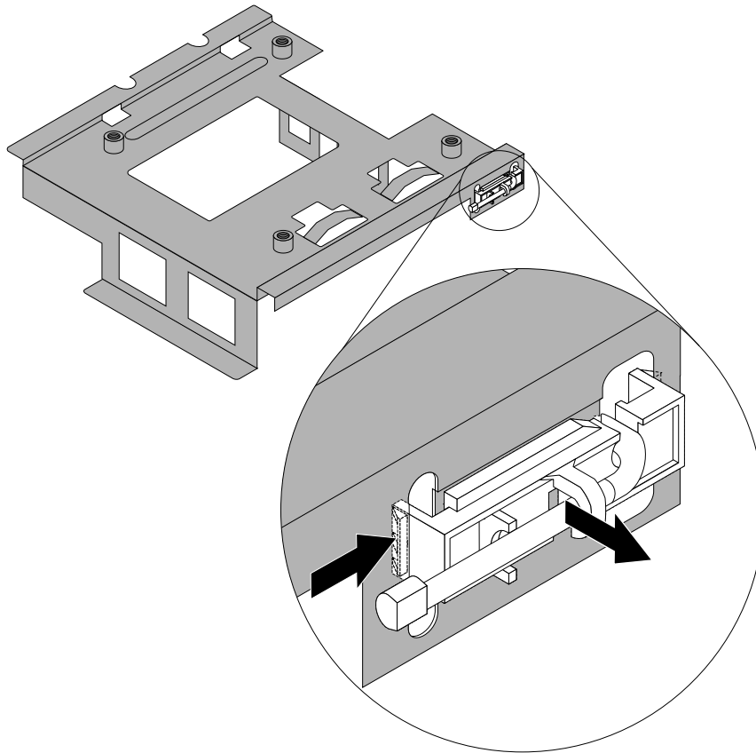
Figure 32. Removing the thermal sensor
