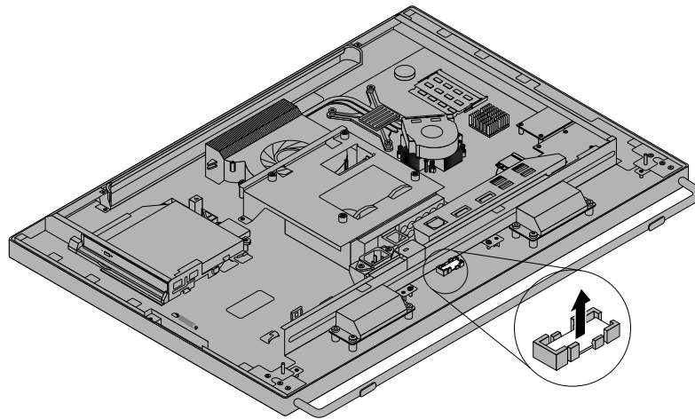
Figure 38. Removing the Bluetooth module
