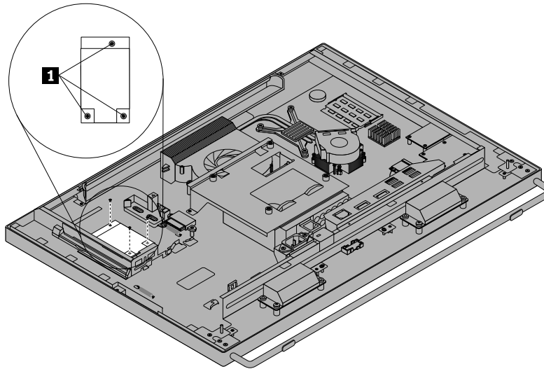
Figure 25. Removing the converter board
