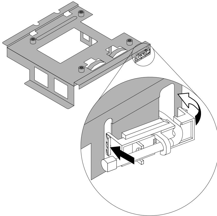
Figure 33. Installing the thermal sensor
