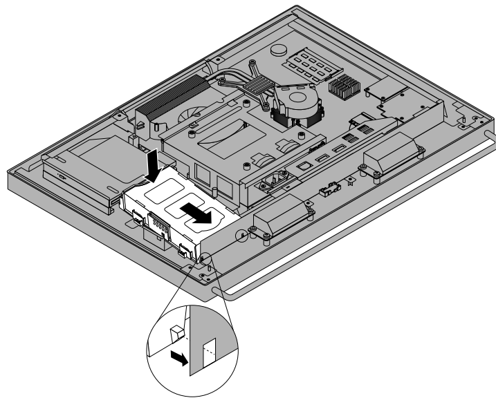
Figure 21. Installing the hard disk drive (20-inch display)
