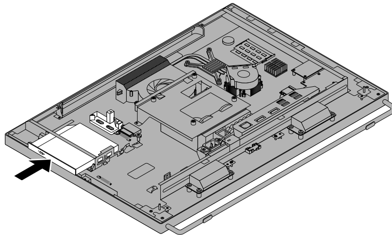
Figure 24. Installing the optical drive
