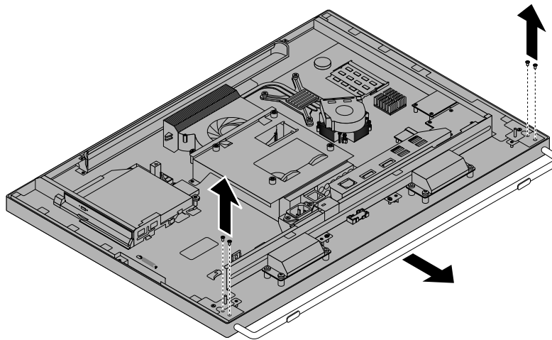
Figure 13. Removing the frame foot
