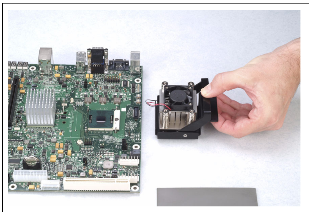
Figure 9. Squeezing Activation Arm
