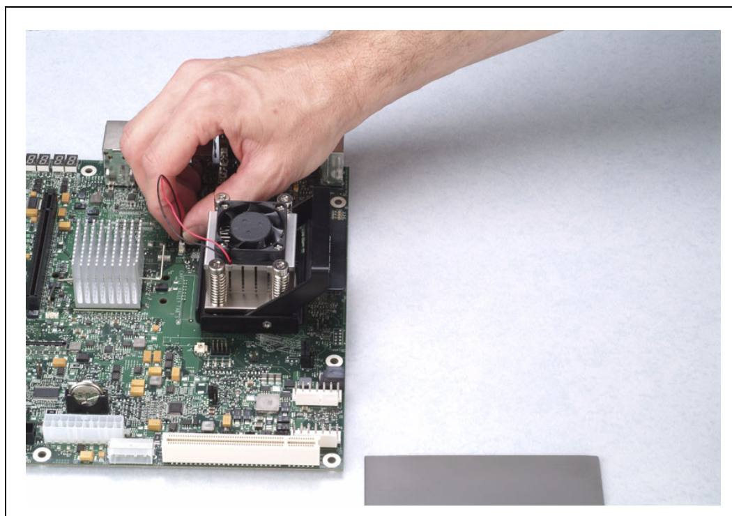
Figure 12. Completed Assembly
