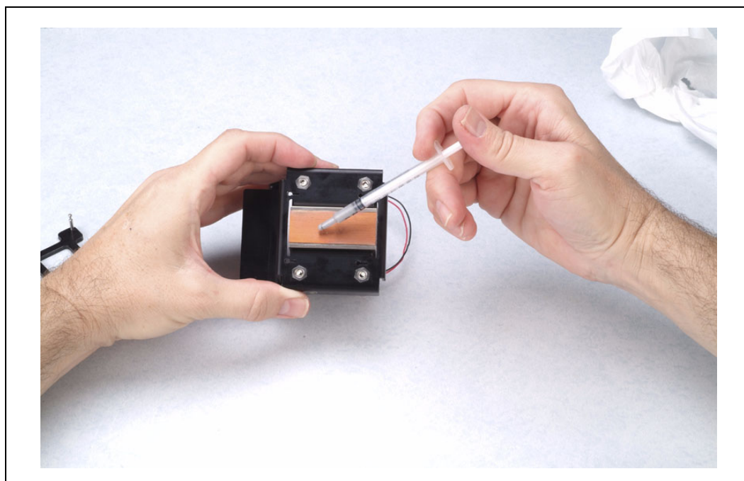
Figure 8. Applying the Thermal Grease
