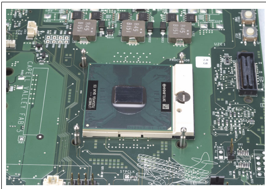
Figure 7. Backplate Pins
