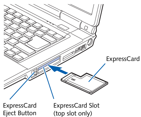
Figure 4-8. inserting/Removing ExpressCards
