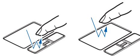
Figure 2-12 Double-clicking methods
