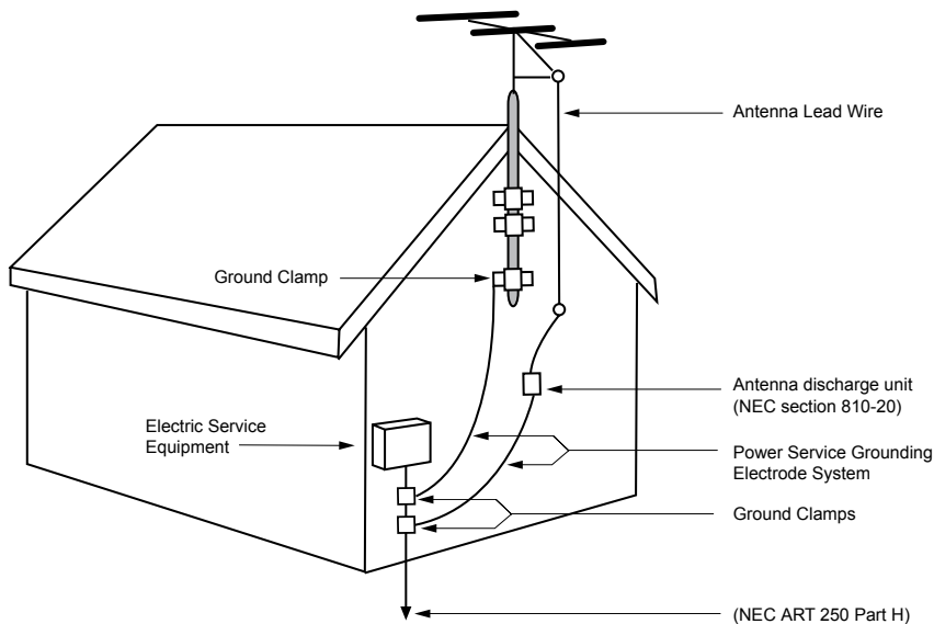
Example of Antenna Grounding
