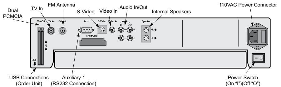
Rear Panel of the DKEC
