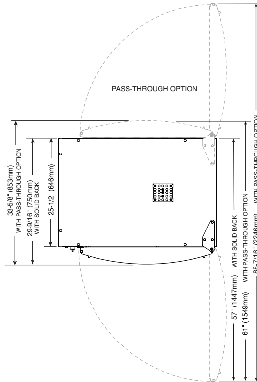
AR-7VH VENTLESS HOOD INSTALLED DIRECTLY ON THE TOP OF ELECTRIC ROTISSERIE MODEL AR-7E
