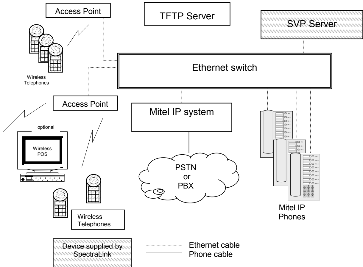
(Mitel Networks IP telephony server architecture example)
