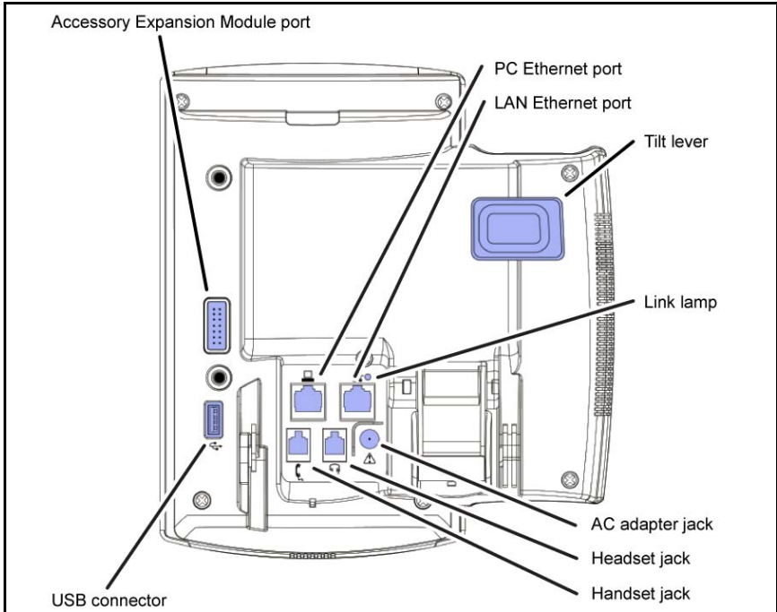
Figure 4: IP Phone 1140E connections
