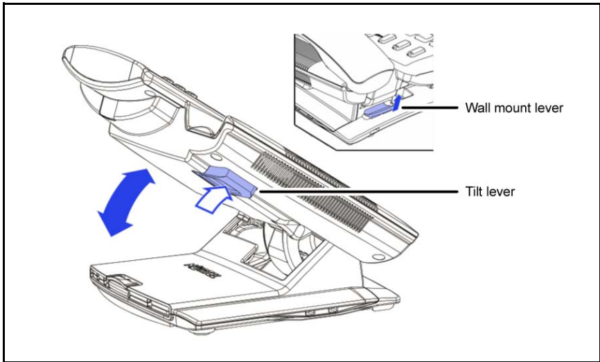
Figure 5: Release the IP Phone 1140E from the stand
