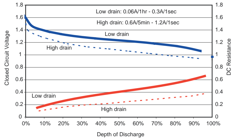
TYPICAL DC RESISTANCE CHARACTERISTICS
