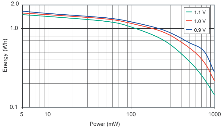
TYPICAL DELIVERED ENERGY VS POWER DRAIN
