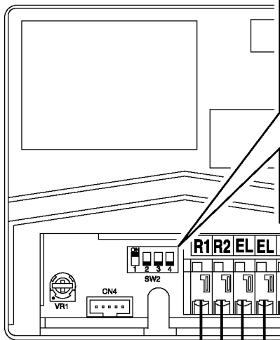
(Entrance station #1) GF-DA Speech Module Back view
