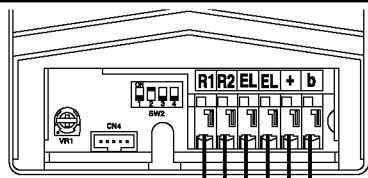
(Entrance station #2) GF-DA Speech Module Back view
