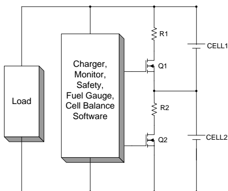
Figure 1. Cell-Balancing Technique Schematic
