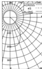
Candlepower Curve
