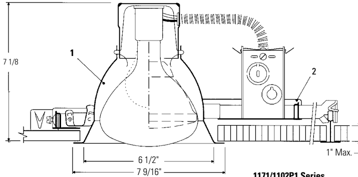
1171/1102P1 Series Standard Incandescent
