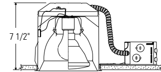
1171/1104ICR Lytefning ™ Convertible Remodeler IC/Non-IC
