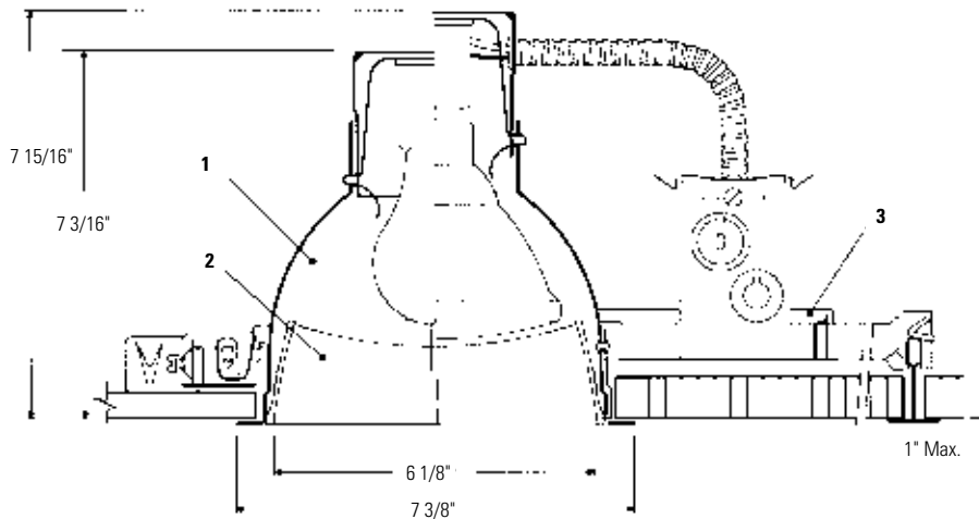
1132/1102P1 Series Standard Incandescent
