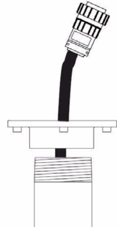
Figure 12. Installing the TLS-300 through the mounting pipe and flange.
