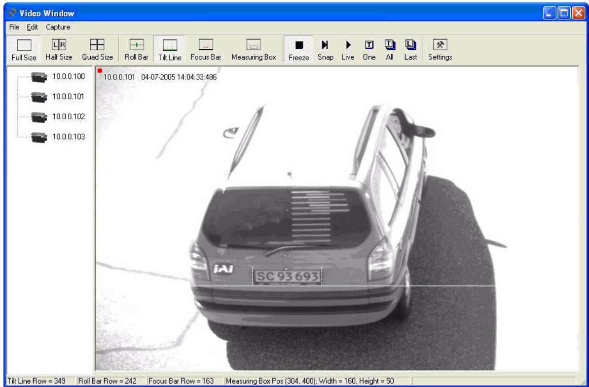
Figure 31. Initial Camera Alignment Display example.
