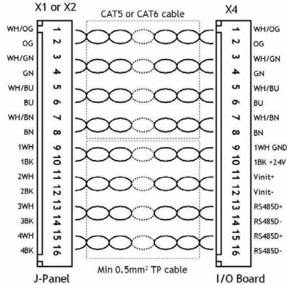
Figure 43. Category 5 or 6 wiring diagram.
