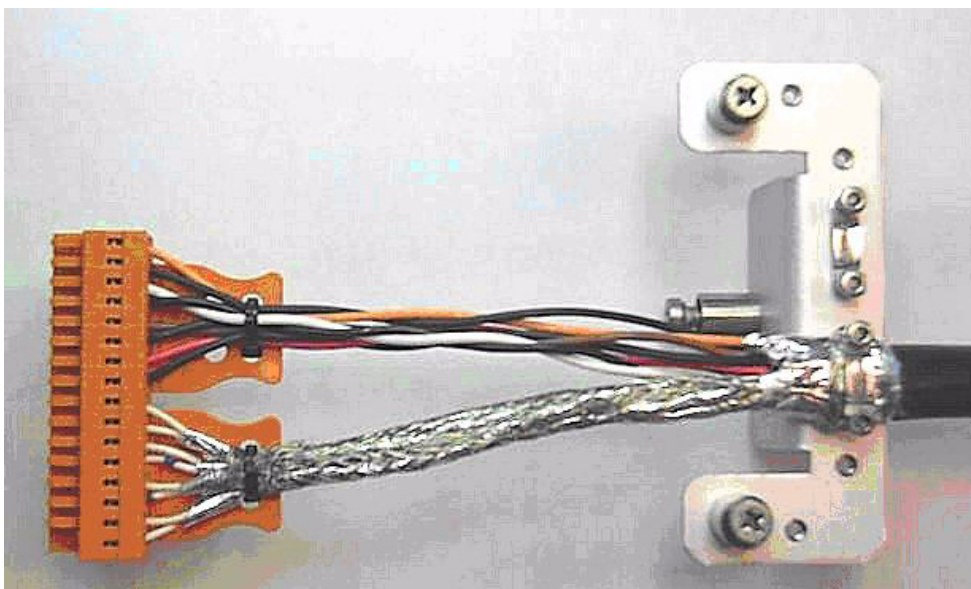
Figure 17. Cable final wiring.
