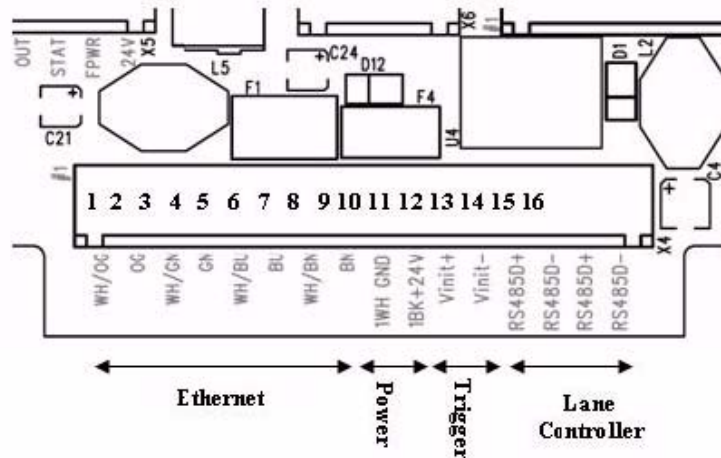
Figure 39. Board connections
