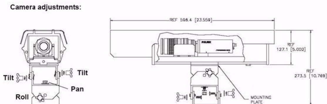
Figure 14. Camera Installation
