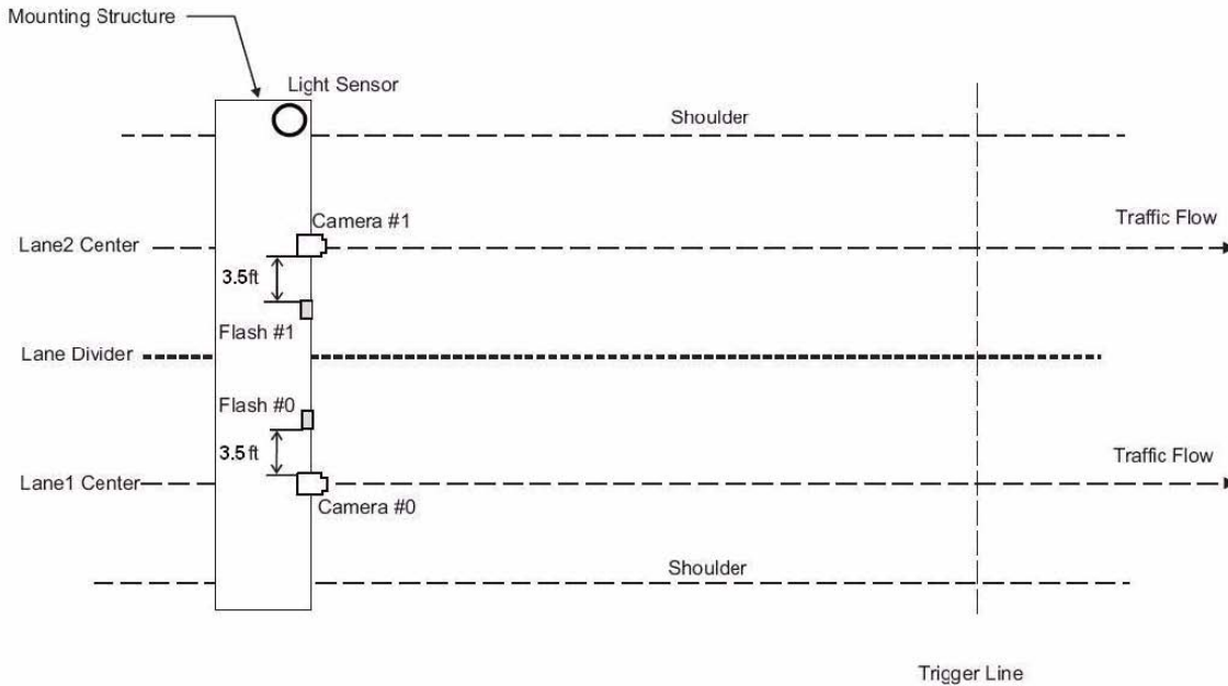
Figure 4. Typical Over Lane Site Layout Plan.
