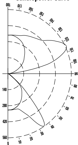
Candlepower Curve
