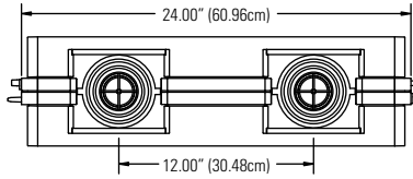
2 Light MR16
