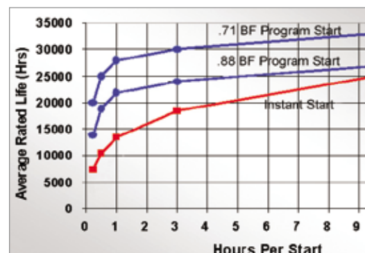
Lamp Life Table using program start and instant start ballasts.
