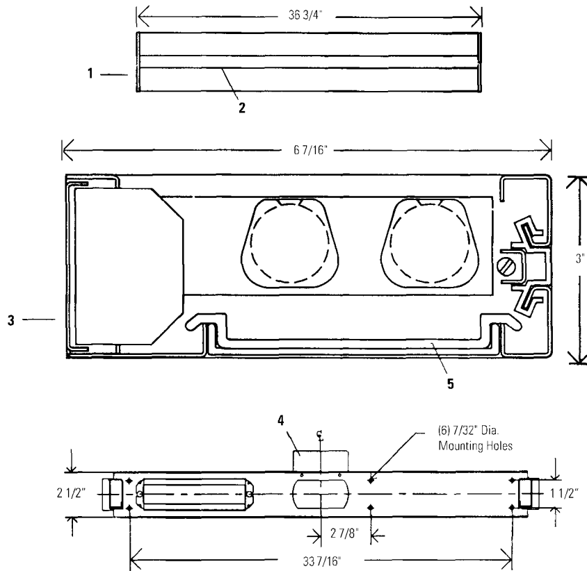
Mounting Plate Assembly
