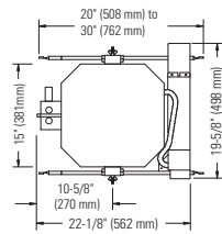
Top View (Magnetic Ballast)
