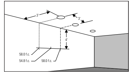
Lighting Data - Example C6P38MHLCLW illumination on the wall 4' down from the ceiling is 58.0 f.c. beneath and 54.8 f.c. between fixtures.
