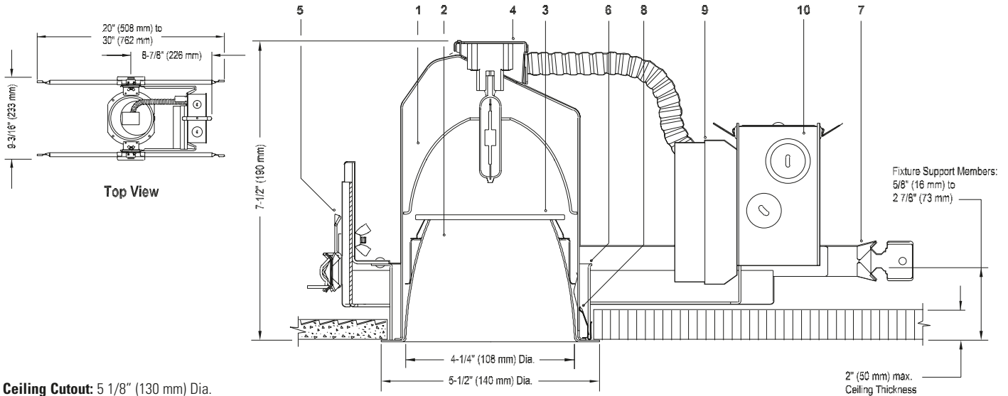
Ceiling Cutout: 5 1/8" (130 mm) Dia.
