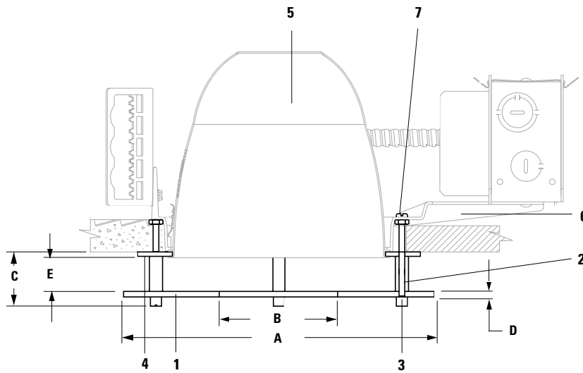
Perforated Metal Disc
